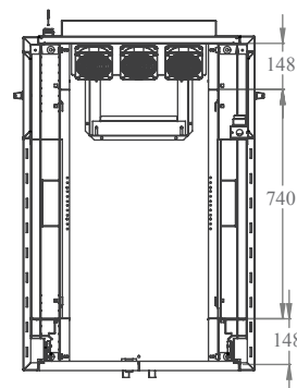
EQUIPMENT MOUNTING DISTANCE
