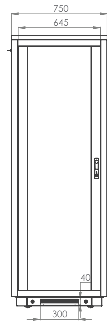
REAR VIEW
