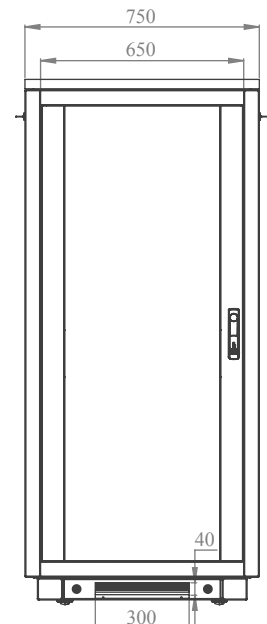
REAR VIEW
