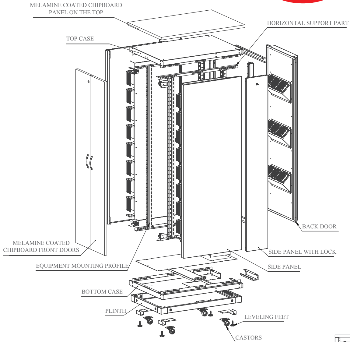
EXPLODED VIEW
