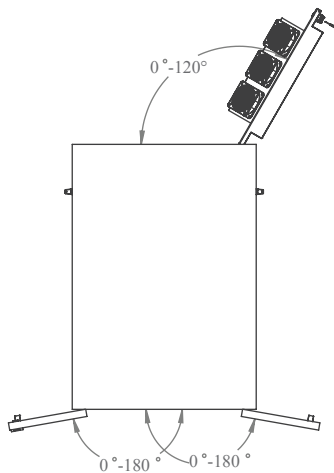
FRONT DOOR OPENING ANGLE
