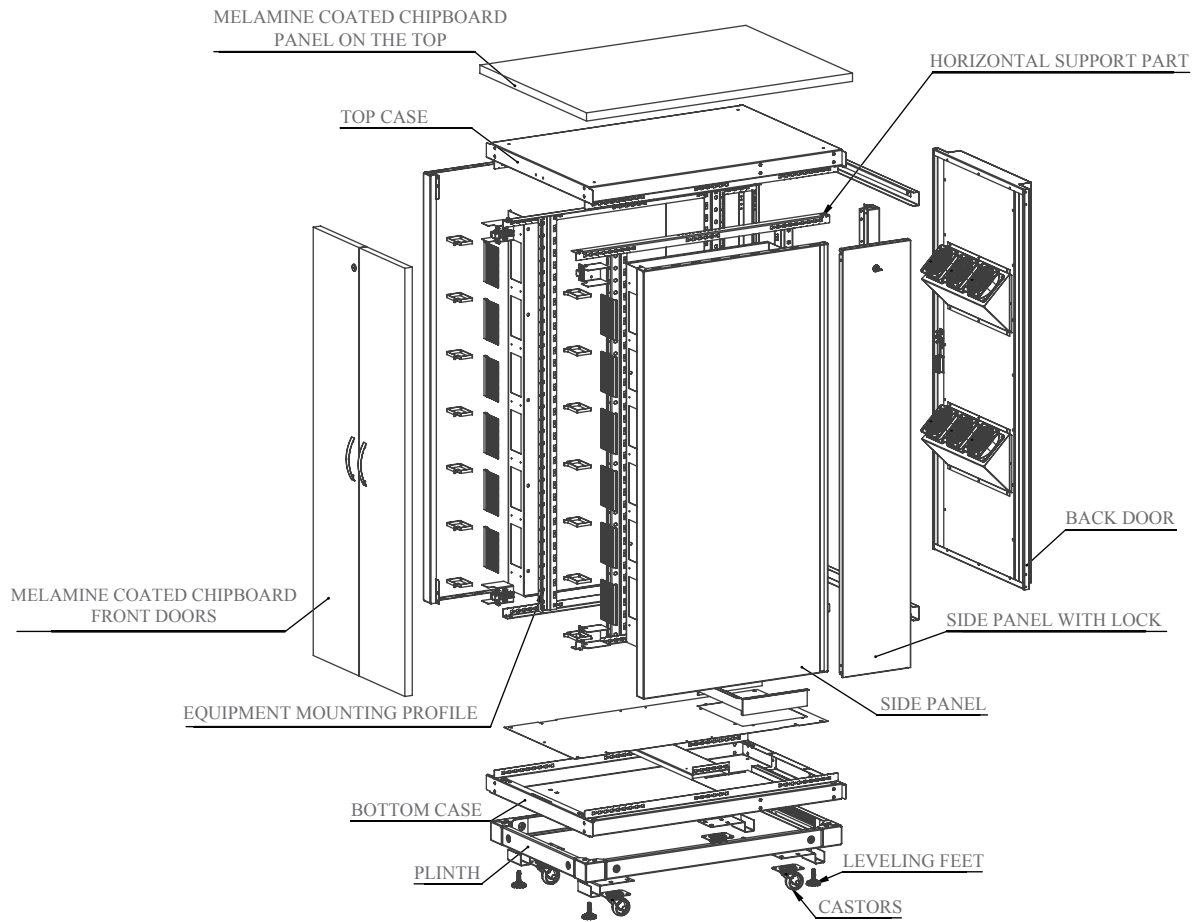
EXPLODED VIEW
