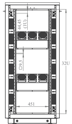
DIMENSIONS IN WIDTH AND HEIGHT
