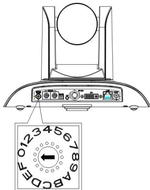
Figure 2.6 Rotary Dial diagram
