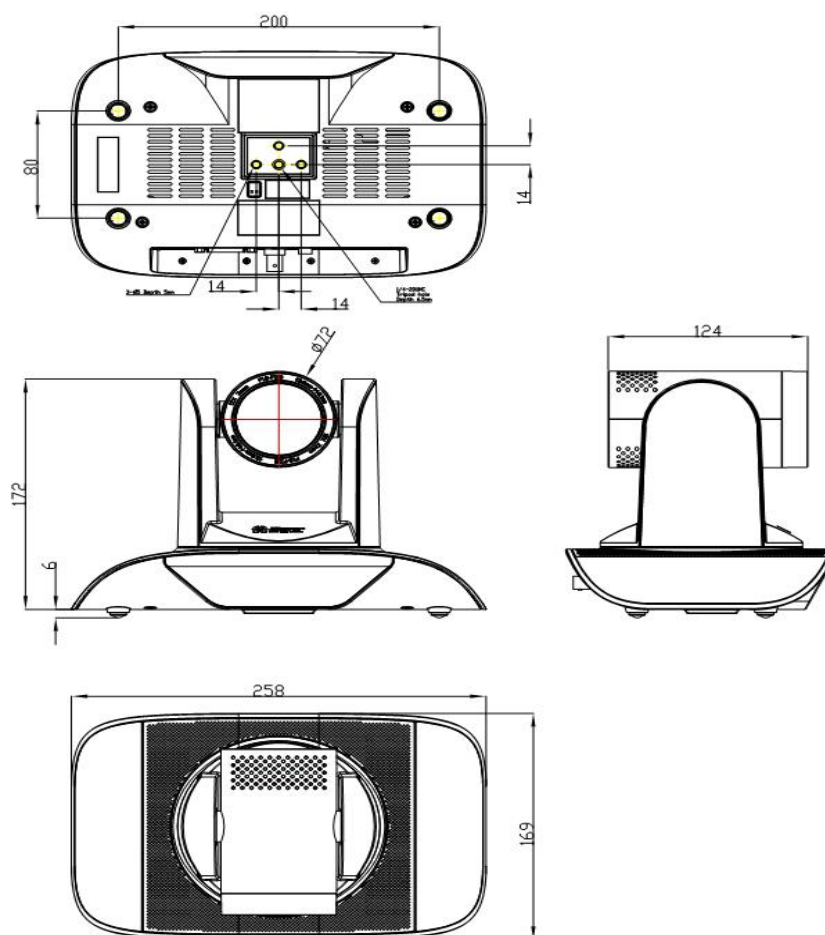
Figure 2.1 Camera dimension
