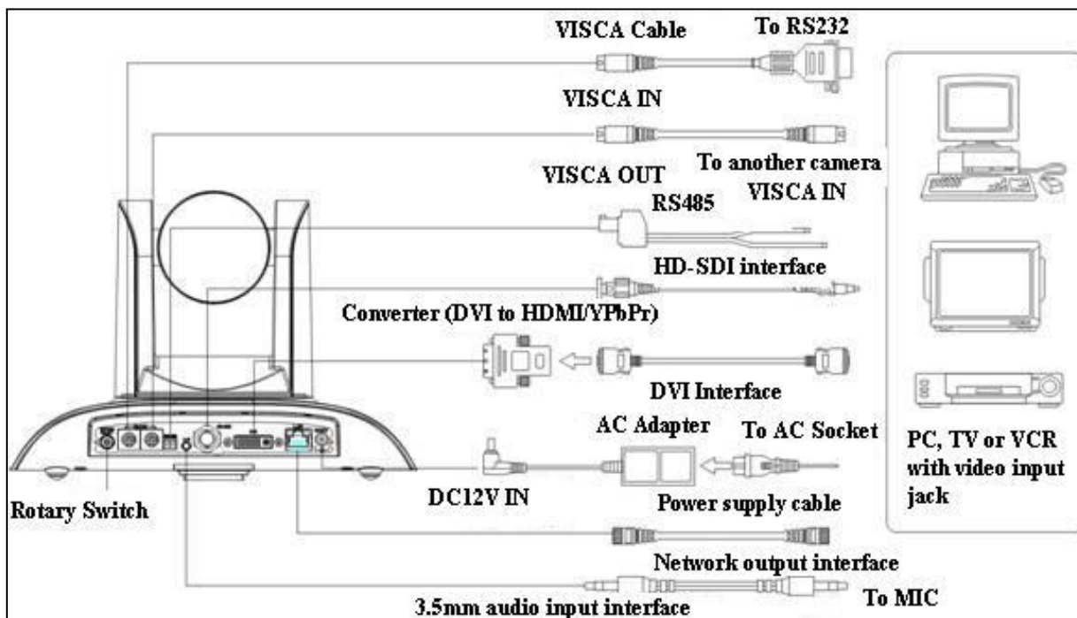
Figure 2.3 model external interface diagram
